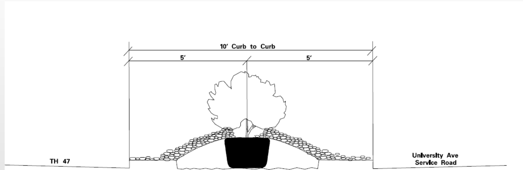
Typical Section Median Planting
